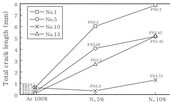
Fig. 4 The effect of shielding gas on total crack length of specimen No.1,5,10 and 13 ( \epsilon=2.52\% )
