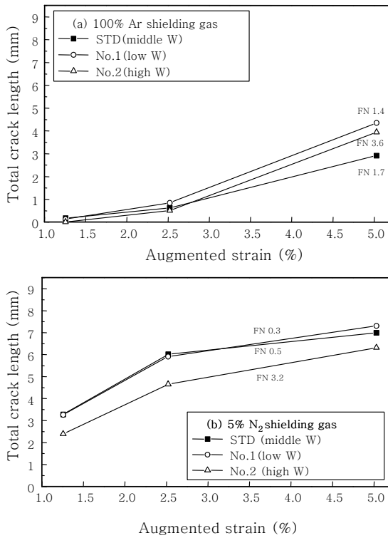
Fig. 5 Total crack length of specimen STD, No.1 and 2
