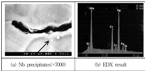
Fig. 15 SEM photos of crack and Nb precipitates and EDX result
