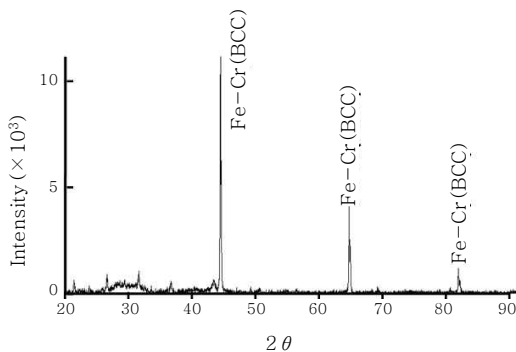
Fig. 7 XRD result of electro-extracted phase
