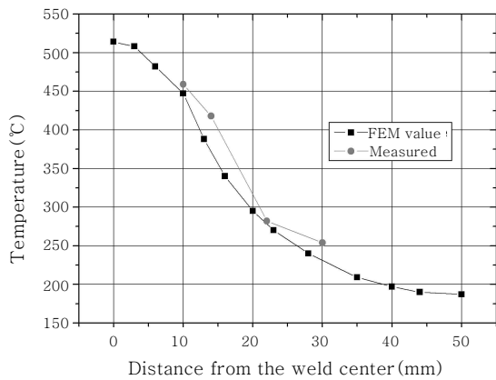
Fig. 14 Measured 1) and calculated temperature profile along the cross section per perpendicular to the weld line for the location 1.6 mm below the top surface when the tool is at the middle point of the plate
