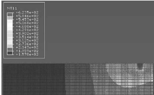
Fig. 11 Temperature field distribution at 94s
