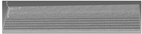
Fig. 2 Three dimensional finite element model and coordinate system
