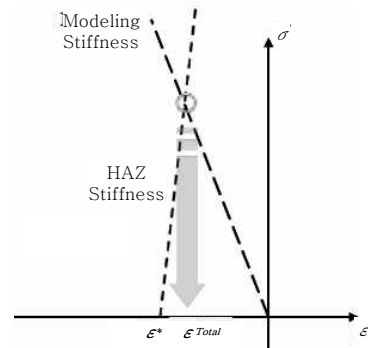
(a) Elastic analysis based on inherent strain
