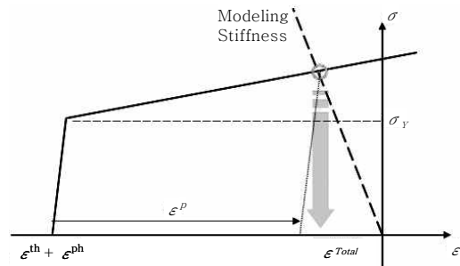
(b) EP analysis based on thermal strain
