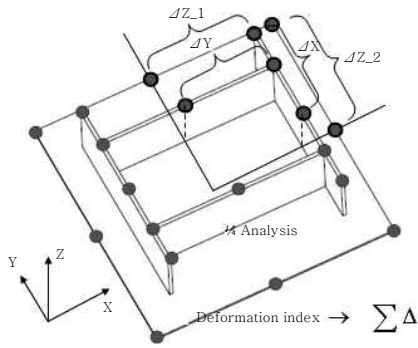
Fig. 5 Deformation index for comparison
