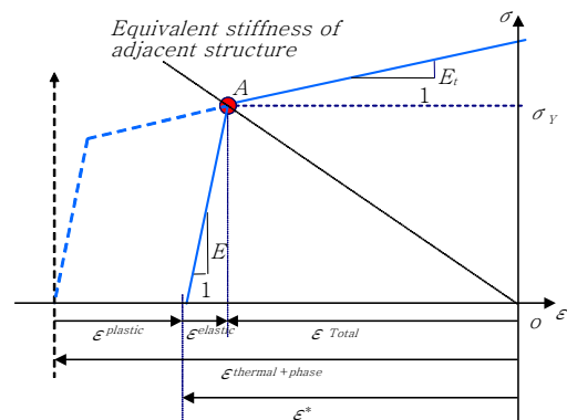
Fig. 1 Inherent strain in stress-strain curve
