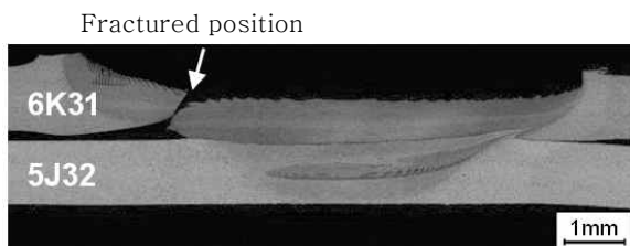
Fig. 9 Typical cross section of fractured specimen
