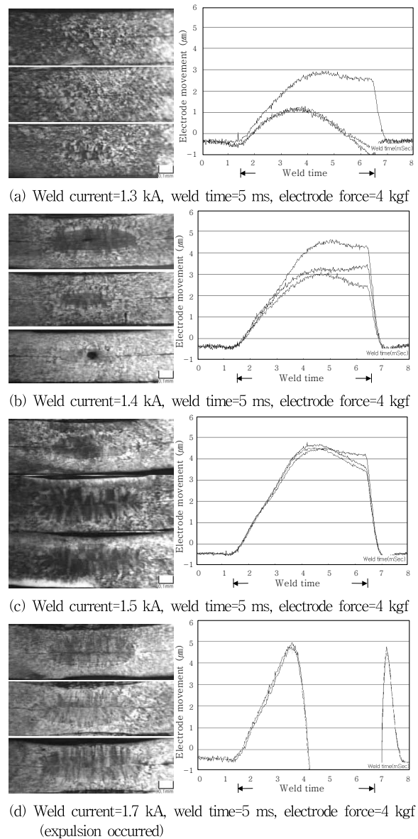
Fig. 7 Photographs of cross-sectioned weldment and corresponding electrode movement
