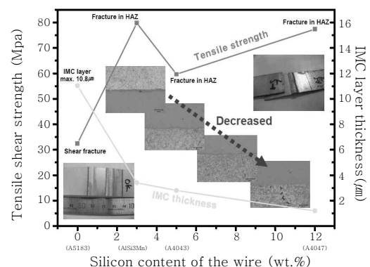
Fig. 5 Build up of IMP, which is strongly influenced by silicon content
