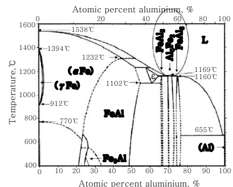
Fig. 2 Fe-Al equilibrium phase diagram
