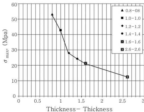
Fig. 5 Relationship between maximum principle stress and plate thickness
