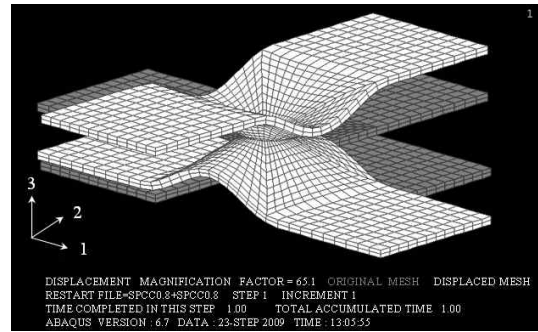
(a) Deformation of [SPCC(0.8)+SPCC(0.8), Ø5.0] spot welded lap joint subjected tensile load
