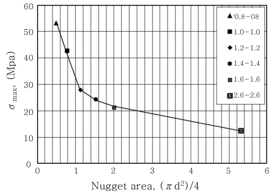
Fig. 6 Relationship between maximum principle stress and nugget area
