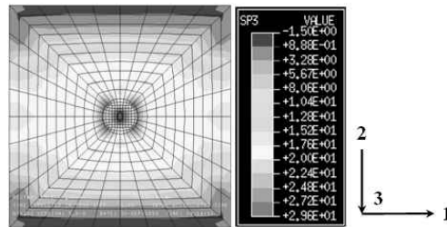
(b) Stress distribution around the nugget on the inner surface
