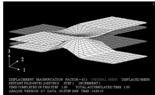
(a) Deformation of [SPCE(1.2)+SPCE(0.8), Ø5.0] spot welded lap joint subjected tensile load
