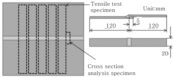
Fig. 2 Schematic illustration of making specimens
