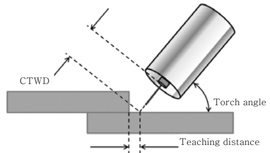
Fig. 1 welding conditions
