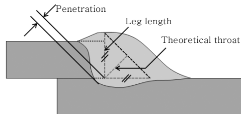
Fig. 3 KS standard geometry factors
