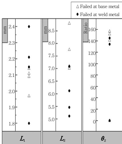
Fig. 9 Results of analysis on additional geometry factors
