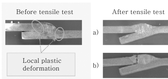
Fig. 5 Results of tensile test (No. 5) a) Failed at base metal b) Failed at weld metal
