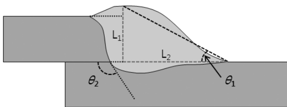
Fig. 8 Additional geometry factors
