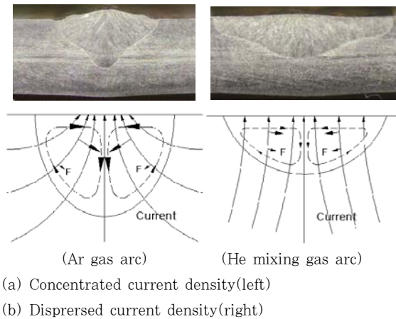
Fig. 7 Lorentz force induced by current density and driving force of molten pool convection
