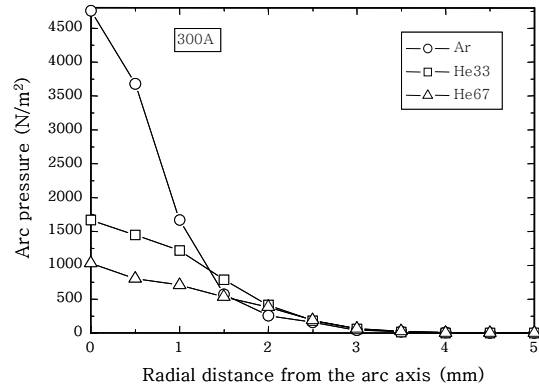
Fig. 2 Arc pressure distribution with the mixing ratio of shield gases
