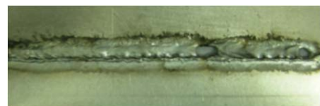
Fig. 5 Bead shape of DC pulse MIG welding
