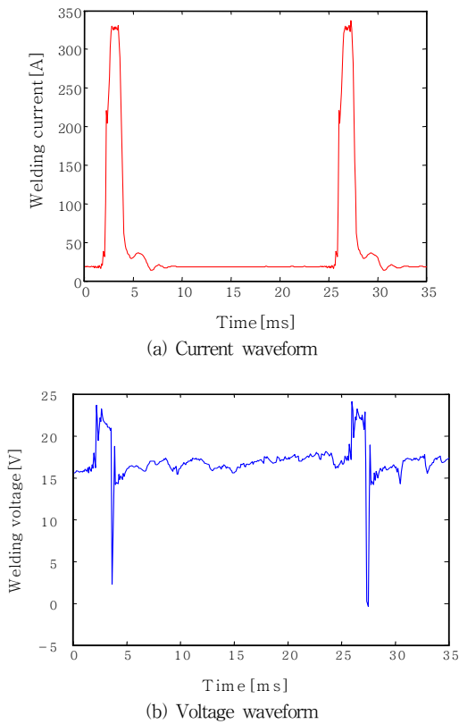
Fig. 6 Current waveform of DC pulse MIG welding
