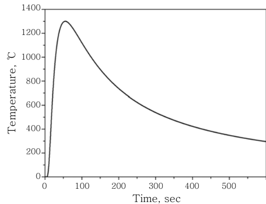
Fig. 1 Thermal cycle for CGHAZ simulation of 500 kJ/cm heat input 6)
