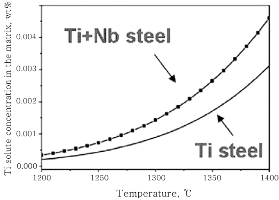
Fig. 11 Solute concentration ( C_m ) of Ti in the matrix c calculated by Thermo-calc 6)
