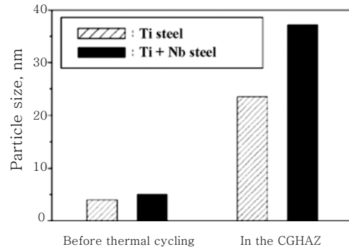
Fig. 8 Particle size of Ti and Ti+Nb steel before and after welding cycle 6)
