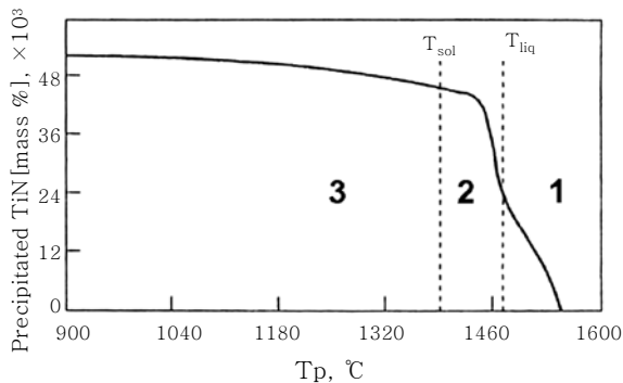
Fig. 3 Progress of TiN for a steel containing 0.8%C, 0.016%N and 0.04%Ti 7)
