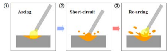
Fig. 8 Three steps of dip-transfer DC GMA welding
