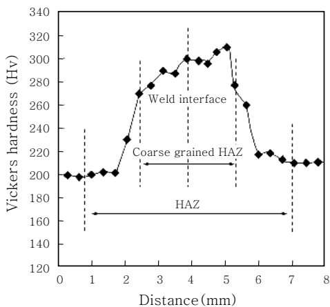
Fig. 5 Hardness distribution of the flash butt welded layer of 590DP steel(As welded)
