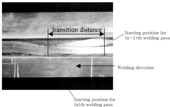
Fig. 11 Transition distance for each welding pass
