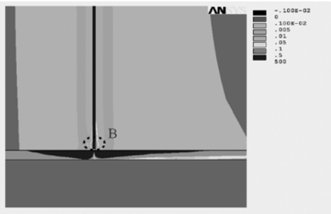
Fig. 6 Contours of magnetic flux distribution
