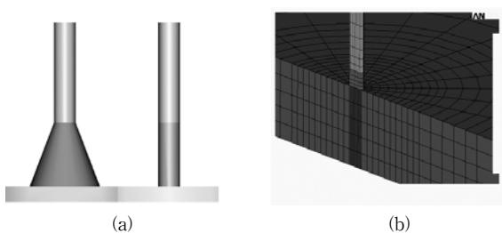
Fig. 4 Configurations of arc and mesh design
