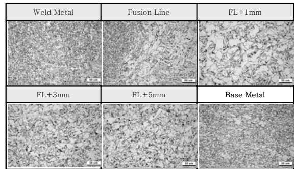
Fig. 7 Microstructure of Tandem EG welded joint
