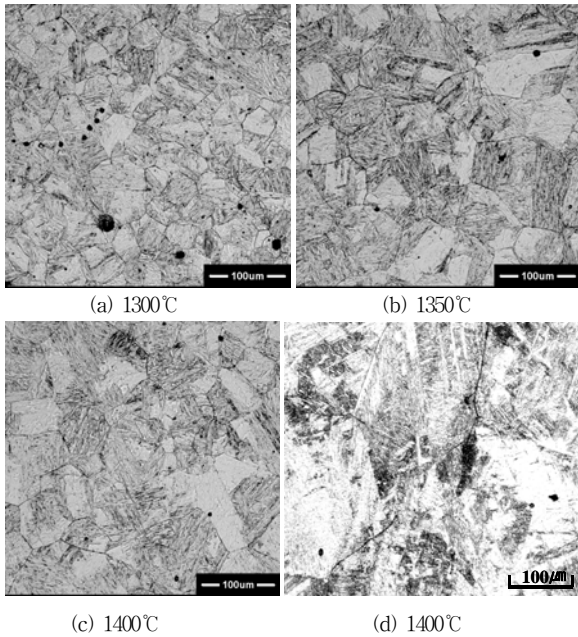
Fig. 4 The microstructure showing austenite grain boundary after heating to peak temperature and quenching a) 1300°C b) 1350°C c) 1400°C in EHB6-TM steel d) 1400°C in conventional TiN steel
