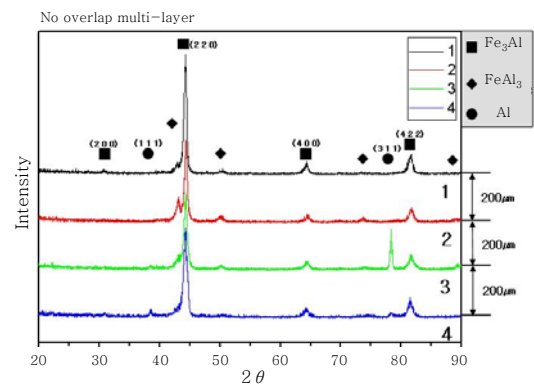
Fig. 13 Phase analysis for no overlap multi-pass overlay
