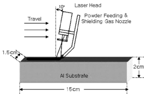
Fig. 1 Diagram of the laser overlay process
