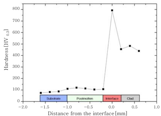
Fig. 9 Micro hardness along the depth of laser overlay
