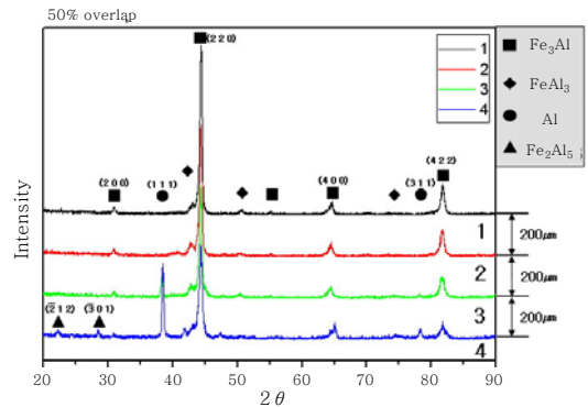
Fig. 12 Phase analysis for 50% overlap multi-pass overlay
