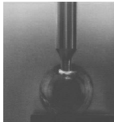
Fig. 6 Thermosonic image of a surface of Al receptacle (measurement I)
