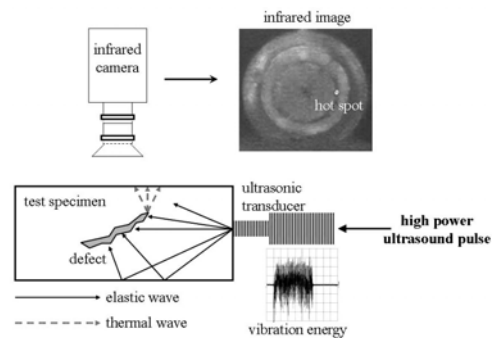
Fig. 1 Principle of ultrasound excited thermography
