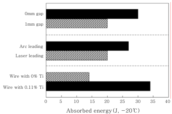
Fig. 7 Effects of hybrid welding conditions on impact toughness of weld metals using side-notched Charpy specimens
