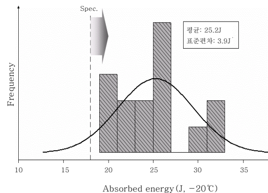
Fig. 13 Absorbed energy for side-notched specimens using new hybrid welding conditions
