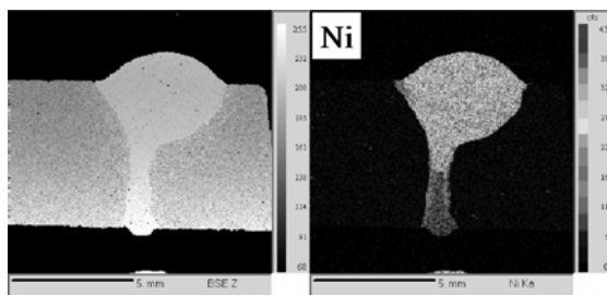
Fig. 5 Distribution of Ni element on hybrid weld metal using EPMA
