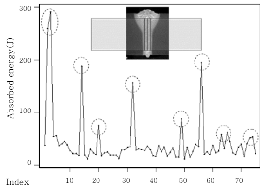
Fig. 2 Result of Charpy impact tests for hybrid weld metals at -20℃
