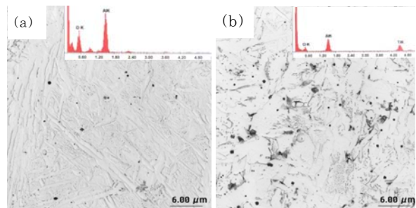
Fig. 10 TEM replicas of weld metals containing (a) <0.003\text{wt.}\%</math> Ti and (b) 0.12wt.% Ti
