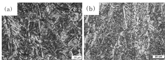
Fig. 9 Microstructure of weld metals containing (a) <0.003\text{wt.}\%</math> Ti and (b) 0.12wt.% Ti
