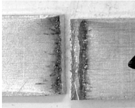
(b) Fracture at weld or HAZ
