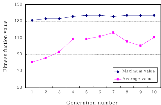
Fig. 6 Best and average values of fitness function in each generation
