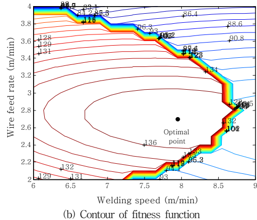
Fig. 7 Fitness function value at 4 kW of laser power
