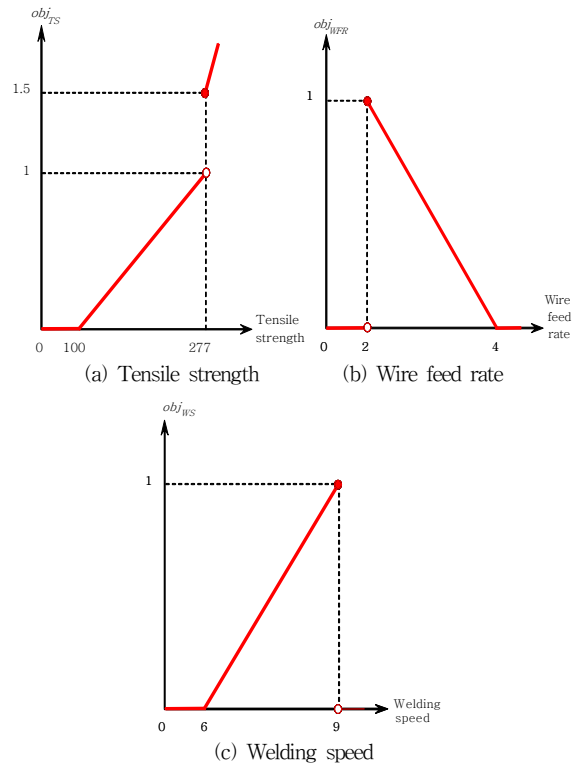
Fig. 4 Objective function
