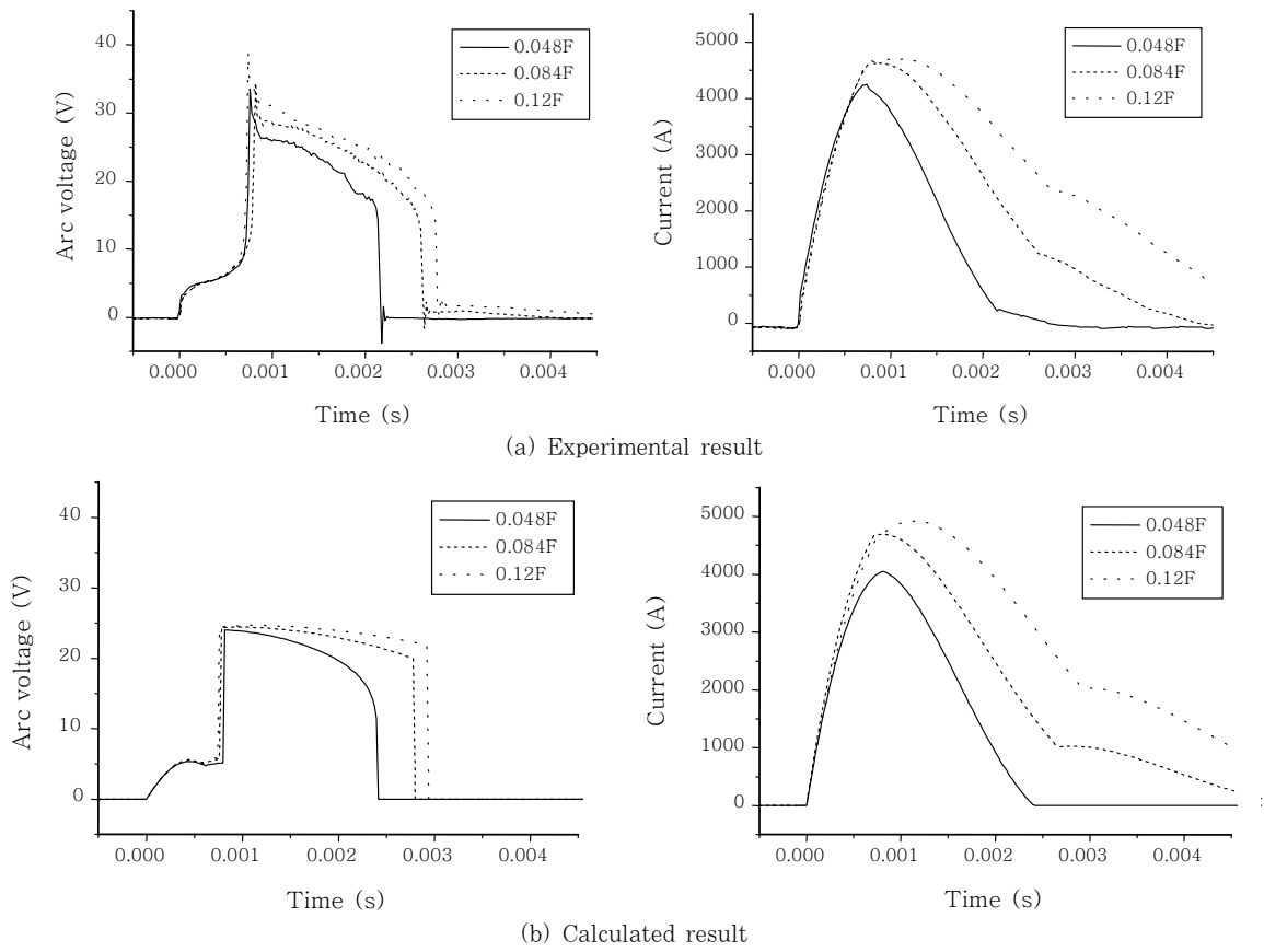
Fig. 10 Effects of capacitance on welding current and voltage
