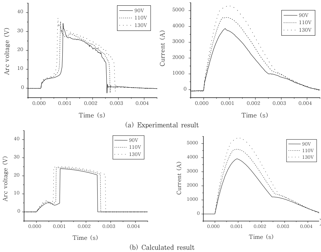
Fig. 11 Effects of charging voltage on welding current
