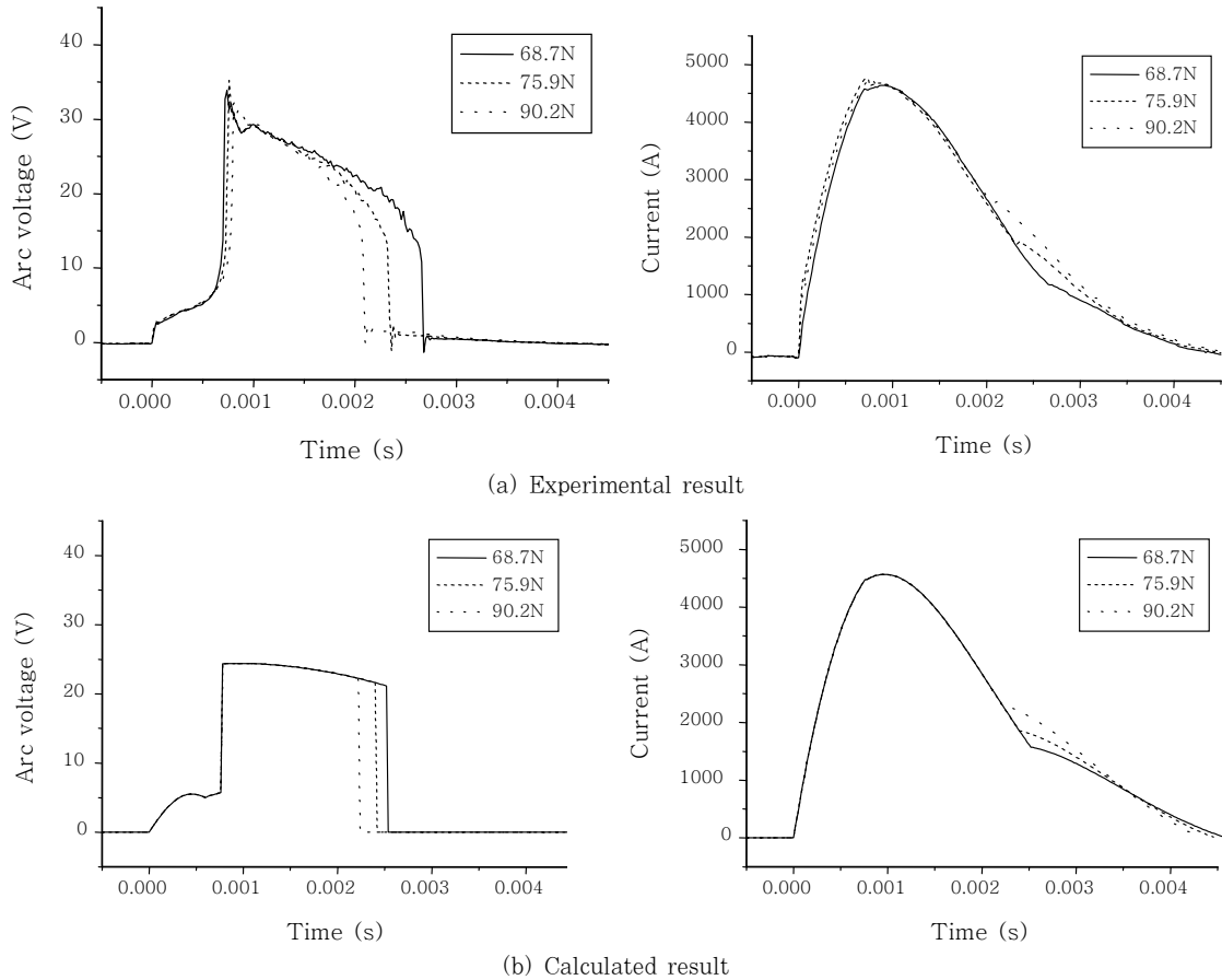
Fig. 12 Effects of spring force on welding current
