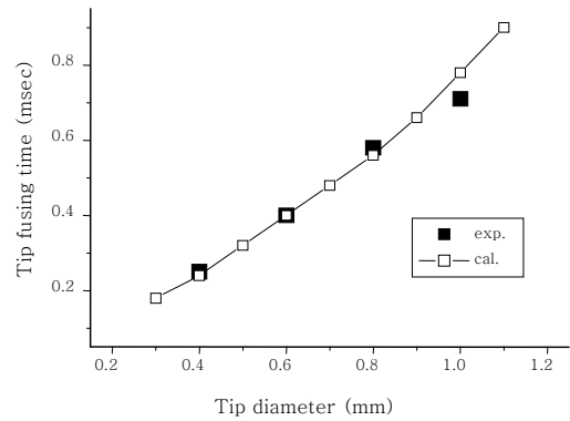
(a) Tip fusing time
