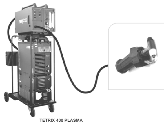
Fig. 6 Equipment for Plasma-Brazing
