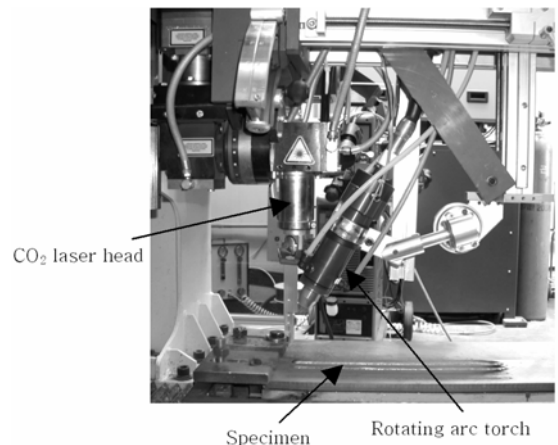
Fig. 2 Photo of laser-rotating arc hybrid welding head
