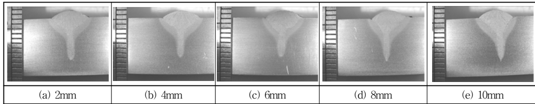
Fig. 7 Cross-sectional bead shapes for various interspacing between laser and center of arc
