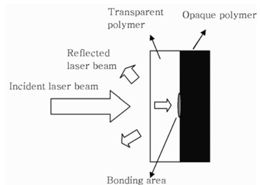
Fig. 3 Schematic diagram of transmission laser bonding
