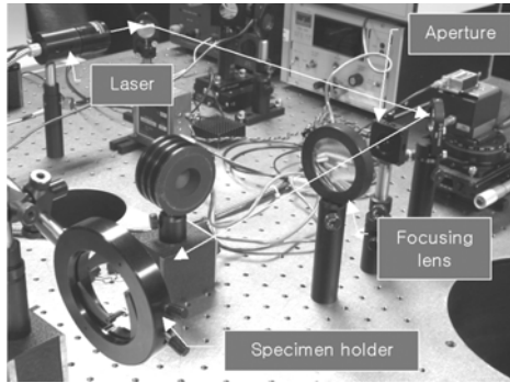
Fig. 6 Experimental setup
