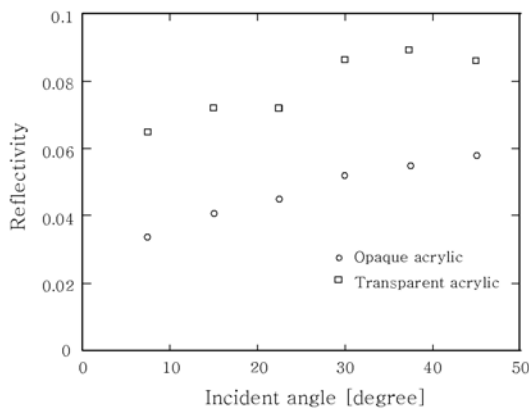
Fig. 4 Reflectivity Vs. incident angle
