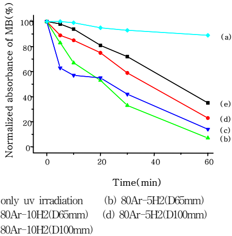
Fig. 8 Photo-decomposition data of TiO 2 coatings using MB solution
