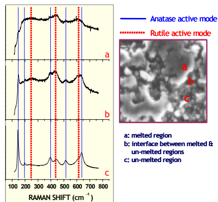
Fig. 7 Raman data of 80Ar-5H 2 (D65mm) coating
