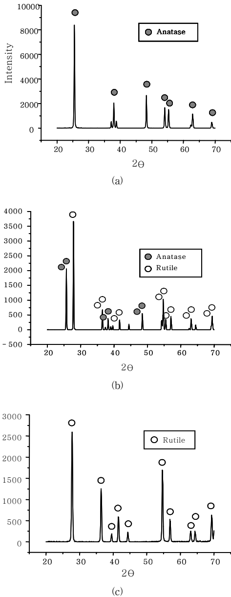
Fig. 10 XRD data of the three TiO 2 pellets formed with different phase-composition (a)100% anatase (b)40% anatase-60% rutile (c) 100% rutile
