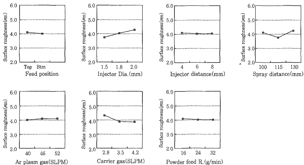
Fig. 4 Effect of the plasma spray conditions on surface roughness
