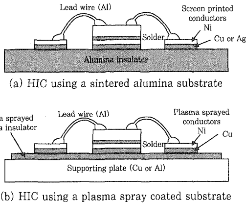
Fig. 1 Schematic comparison of a sintered and plasma spray coated substrate for HIC
