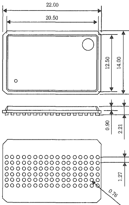
Fig. 1 Overall dimensions of the PBGA
