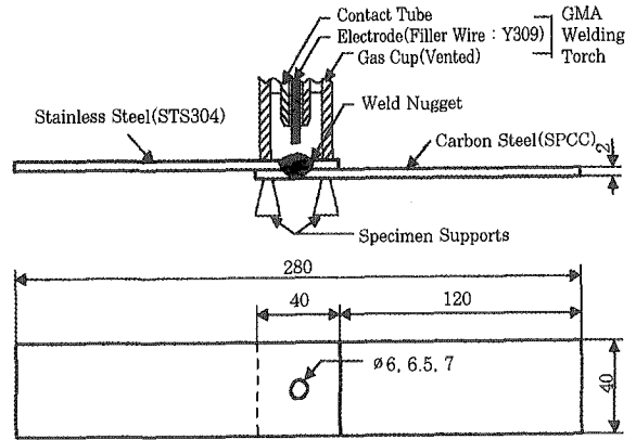
Fig. 1 Specimen configuration and welding setup for arc spot welding process
