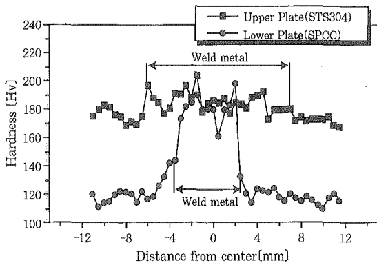
Fig. 5 Distribution of micro-vickers hardness for dissimilar weld metal
