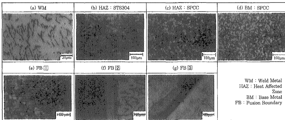
Fig. 4 Microstructure of weld zone
