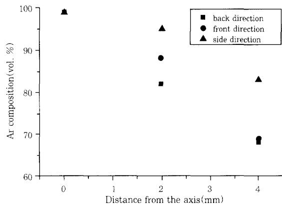
Fig. 12 Ar composition in 3 directions with respect to auxiliary torch (20 liter/min, Ar ratio = 30%, distance from workpiece = 5mm, CTWD=19mm)
