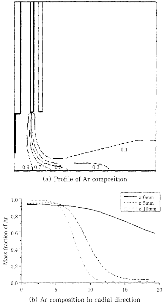
Fig. 6 Distribution of Ar composition for DMAG torch(20 liter/min, Ar ratio = 35%, CTWD = 19mm)
