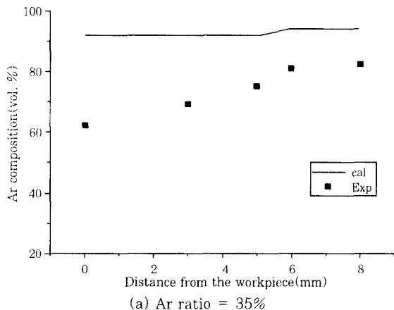
Fig.8 Ar composition in axial direction for DMAG torch
