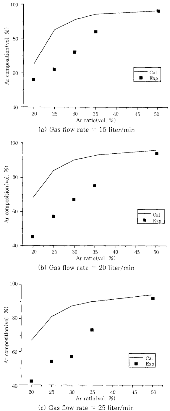
Fig. 7 Effects of gas flow rate on Ar composition at wire tip for DMAG torch(distance from workpiece = 5mm, CTWD = 19mm)
