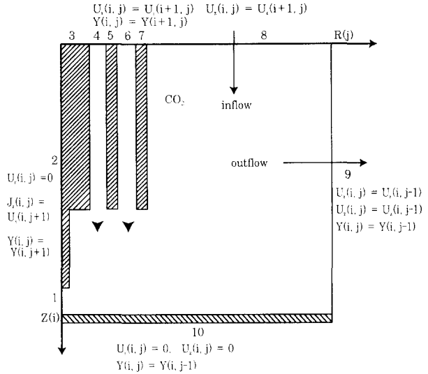
Fig.2 Boundary condition for DMAG torch
