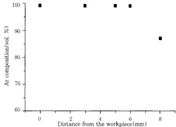
Fig. 11 Ar composition in axial direction for AMAG torch (20 liter/min, Ar ratio = 30%, CTWD = 19mm)
