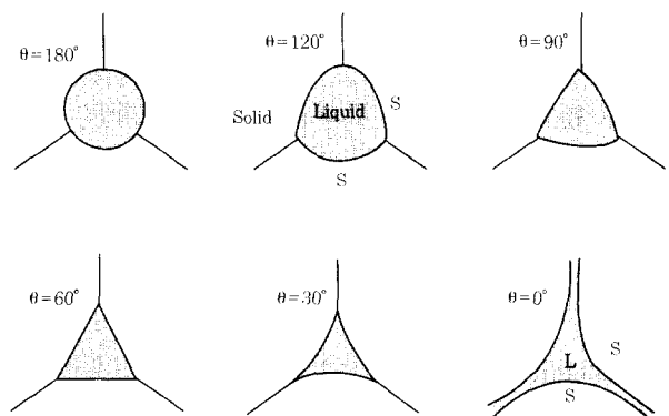
Fig. 7 Dihedral angle of liquid and distribution of liquid during solidification
