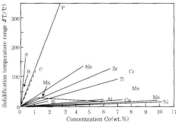
Fig. 6 Effect of solute concentration on solidification temperature range in Fe base-binary system
