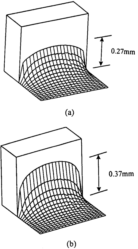
Fig. 4 Calculated solder profiles on the vertical plane (a) no wicking (b) wicking ( Y_w = 25\text{erg/cm}^2 )
