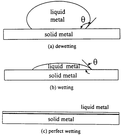
Fig.1 Typical wetting phenomena
