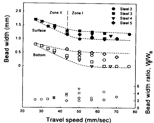
Fig. 5 Effect of travel speed on the bead formation
