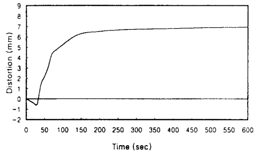
Fig. 8 Angular distortion history at 3rd pass welding in experiment (B point)
