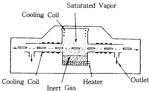
Fig. 5 Configuration of vapor phase soldering type.
