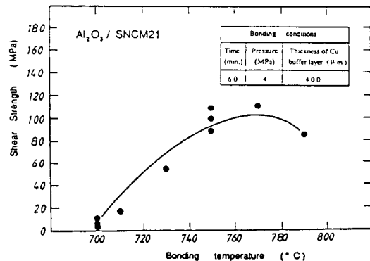
Fig. 3 Dependence of shear strength of \text{Al}_2\text{O}_3/\text{SNCM21} joint on bonding temperature using Ag-Cu-Ti insert metal
