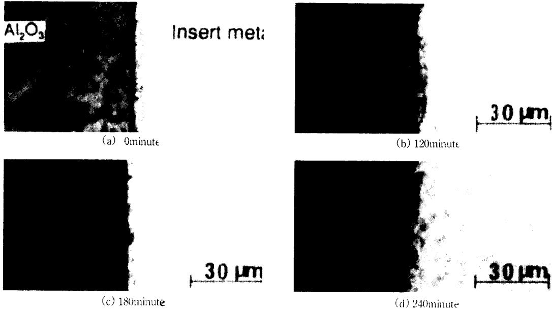
Photo. 2 Microscopic appearance of reaction layer with increasing the holding time (Bonding temperature ; 750/Pressure ; 4MPa)
