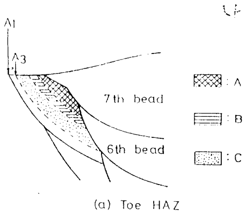
Fig. 1. Welding configuration.
