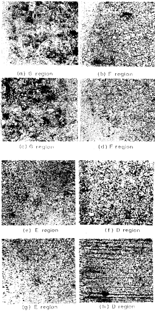
Photo 2. Microstructures of various HAZs in midsection for SS41 and SM53B weldment. (a),(b)SS41 (c),(d)SM53B (e),(f)SS41 (g),(h)SM53B
