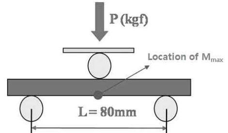
Fig. 3 Schematic of bending test
