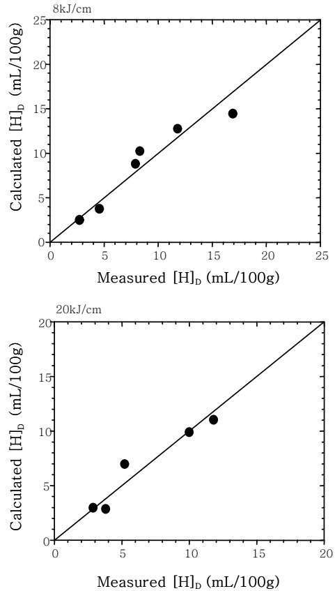
Fig. 7 Comparison between calculated and measured [H]_D in 81T1 wire
