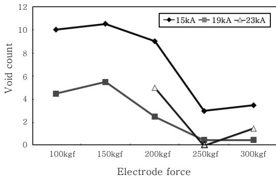
Fig. 11 Variation of void count in nugget (Weld time:100msec)
