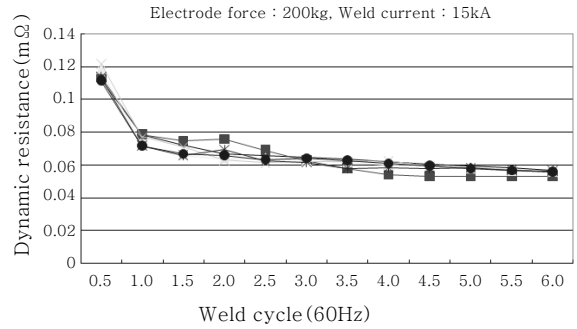
Fig. 4 Typical dynamic resistance patterns
