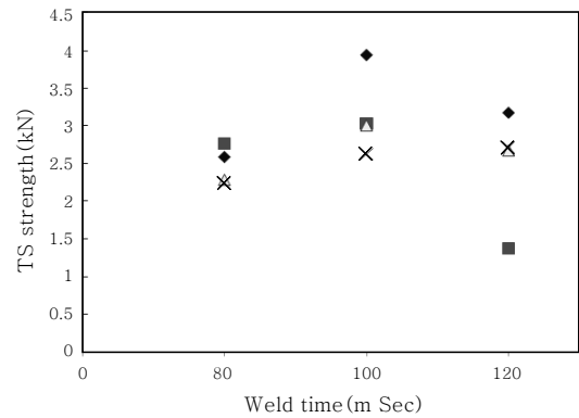
Fig. 8 TS strength vs weld time (Electrode force: 200kgf, Current: 23kA)
