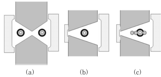
Fig. 7 Variable techniques for consumable guide method ESW. (a) Tandem technique with two consumable guides/electrodes for double V-groove (b) Single electrode method (c) Single electrode wing attached consumable guide method
