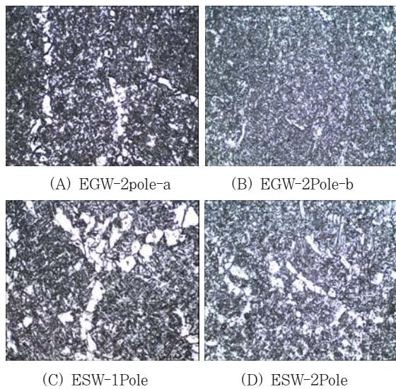
Fig. 10 Microstructure of EGW and ESW - 65mm thick( \times 200 )
