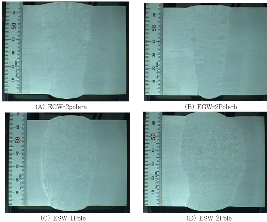
Fig. 9 Macro section of EGW and ESW - 65mm thick
