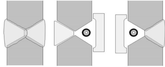
Fig. 6 Two pass welding for double V-groove of consumable guide tube method ESW
