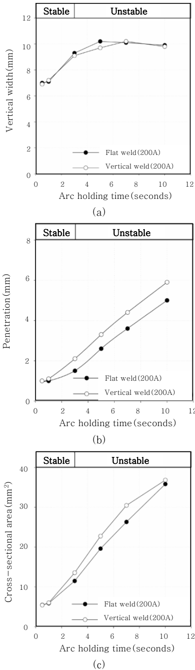
Fig. 3 Measured weld pool (a) width, (b) penetration and (c) cross-sectional area for 200A spot GTAW
