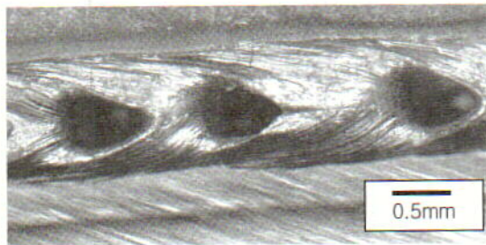
Fig. 4 Typical outer cavities on the laser bead
