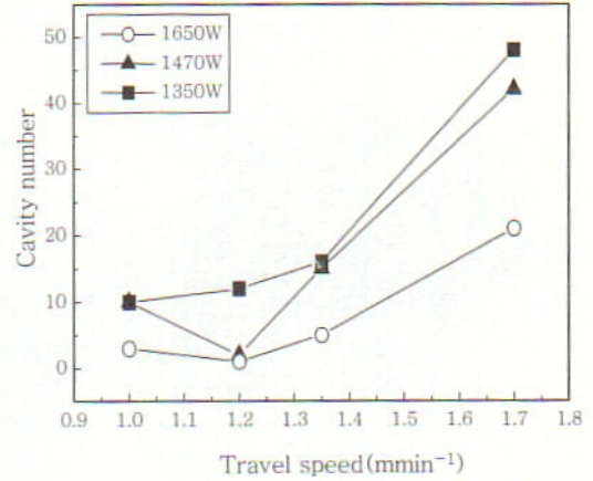
Fig. 5 Relationship between outer cavity and welding parameters
