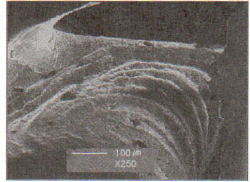
Fig. 8 SEM micrograph of surface of outer cavity
