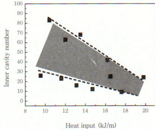
Fig. 10 Effect of heat input on inner cavity formation
