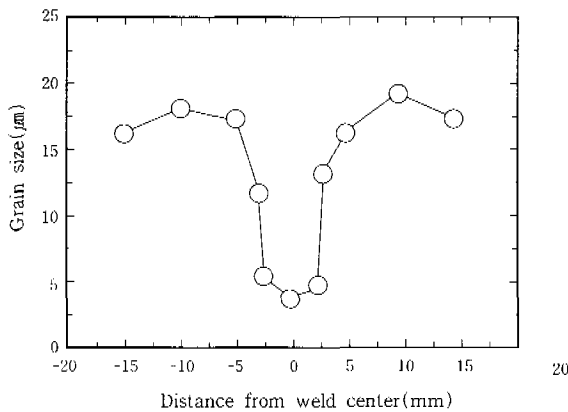
Fig. 8 Grain size distribution in friction-stir-weld of 5083 Al
