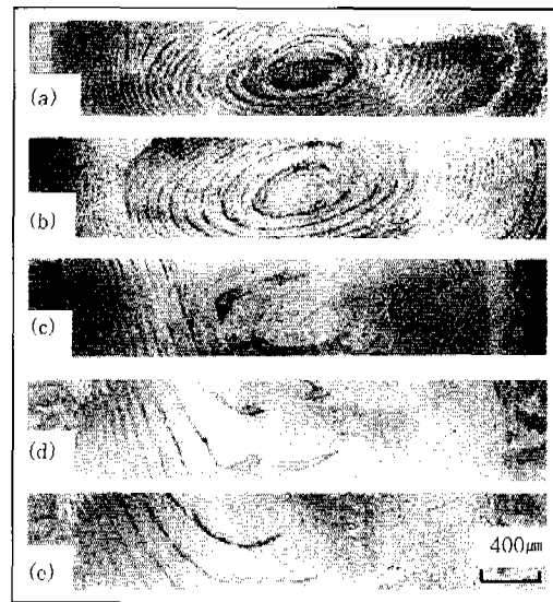
Fig. 5 Transverse cross section of FSW butt joints (5083Al, 4t)with travel speed (a)87 (b)127 (c)187 (d)267 (e)342(mm/min)
