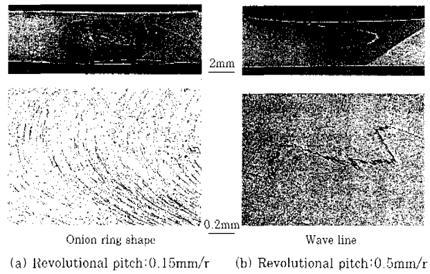
Fig. 13 Optical microscopic observation of oxide at various revolutional pitch
