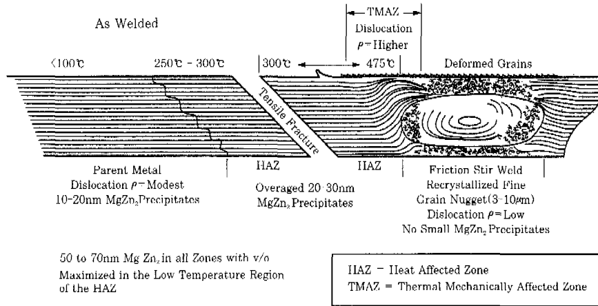
Fig. 10 Schematic illustration of friction-stir-weld zone microstructures, precipitate distributions and temperature ranges for 7075 T651 Al
