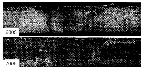
Fig. 2 Cross sectional macrostructure of FSW butt joint
