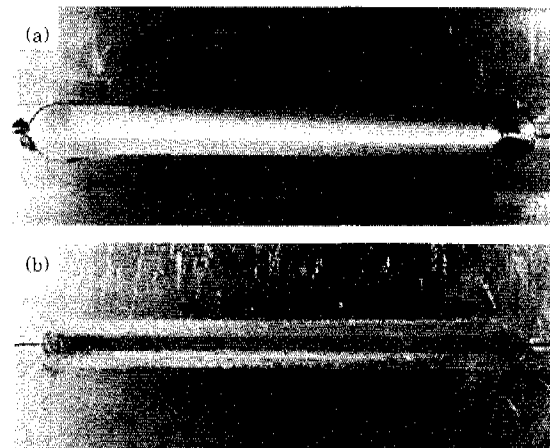
Fig. 1 Surface and back appearance of FSW butt joint(6005Al, 4t)
