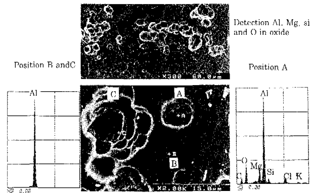
Fig. 14 SEM image and EDX analysis of oxide
