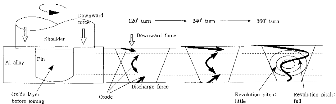
Fig. 15 Growth and stirring model of oxide during FSW
