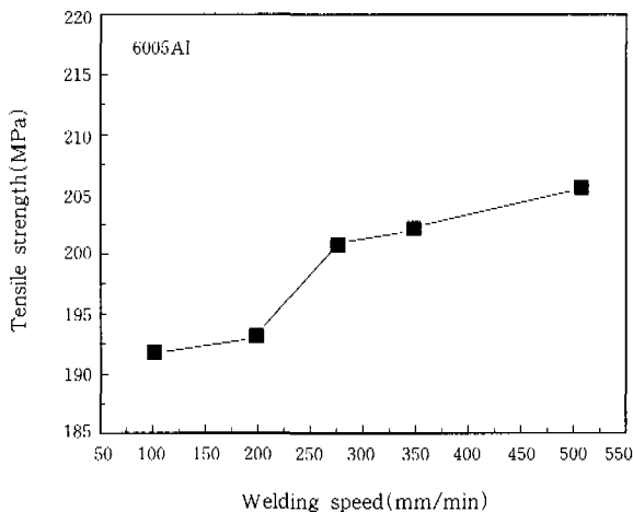
Fig. 17 Effect of welding speed on tensile strength
