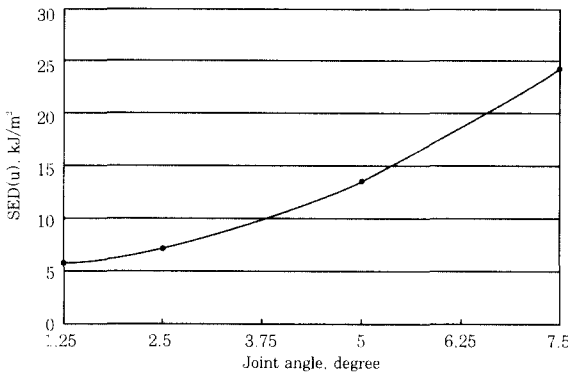
Fig. 9 Relation between strain energy density and joint angle of plate.
