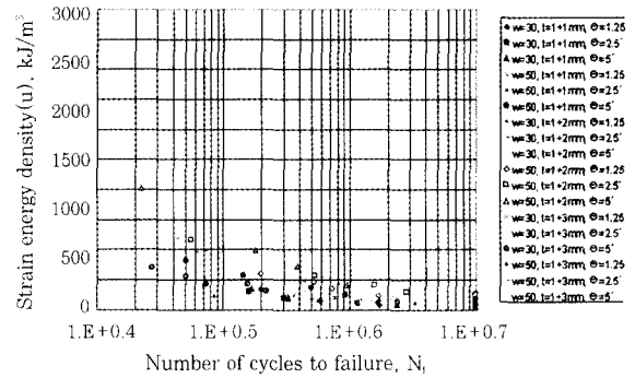
Fig. 11 Relation between \Delta P - N_f
