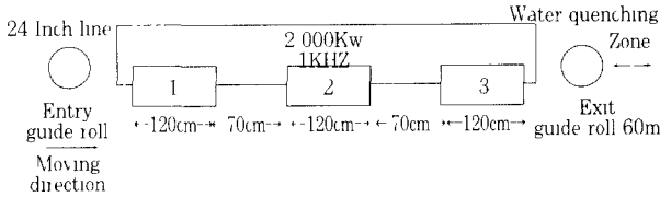
Fig. 4 Inductor arrangement of seam annealer
