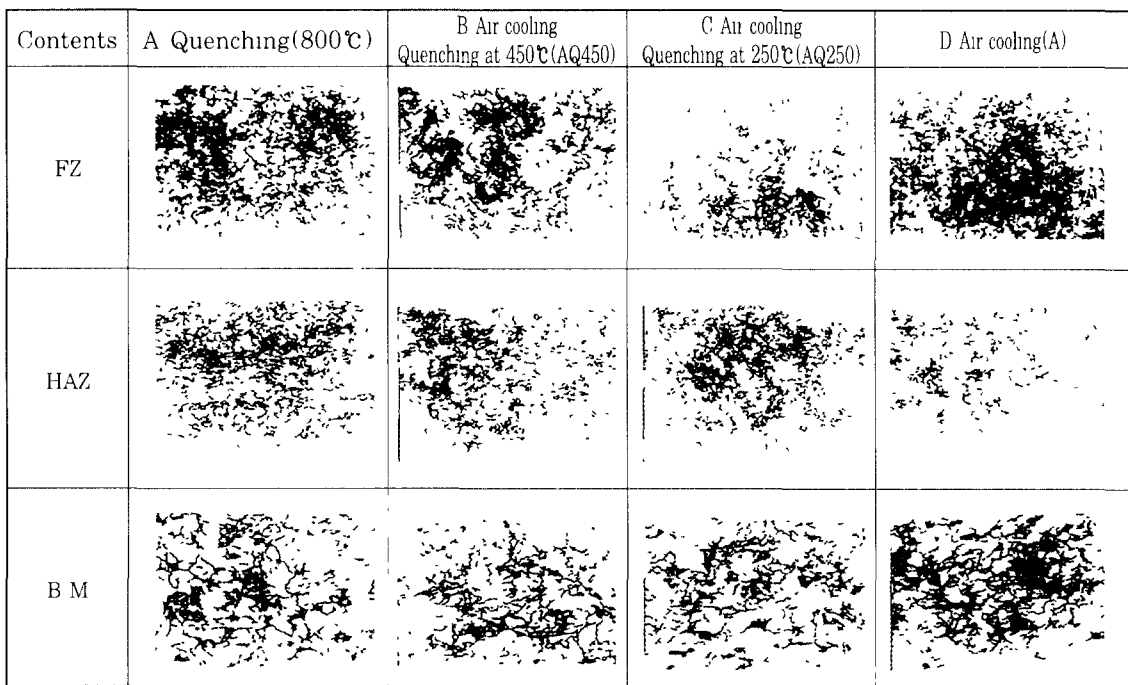
Photo 3. Weld microstructure after heat treatment at 800℃ (X400)
