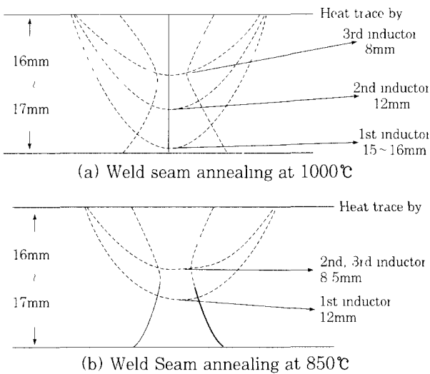
Fig. 10 Penetration depth of heat trace
