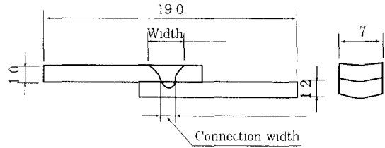
Fig. 1 Geometry of tensile shear test specimen (mm)
