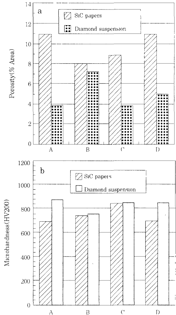
Fig. 2 Property variation from metallographic technique for plasma-sprayed WC-12%Co coatings (a) Porosity and (b) Microhardness Notations for A, B, C, and D represent the coatings produced by different process parameters
