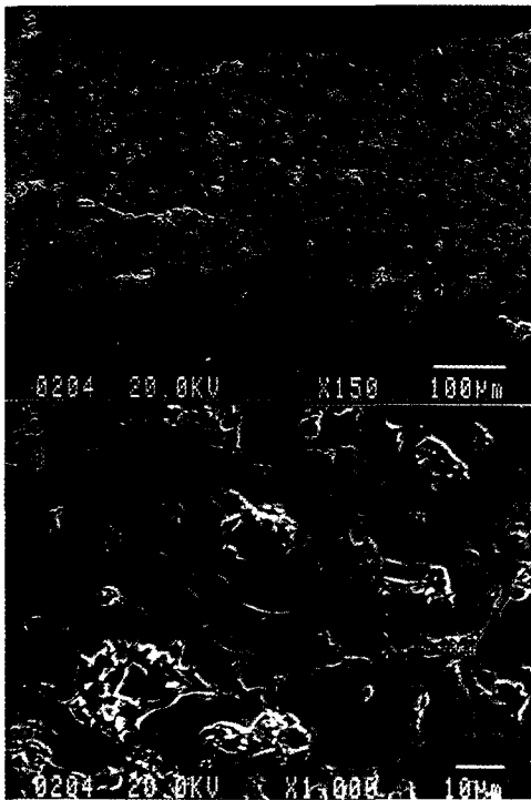
Fig. 1 Typical cross-sectional microstructures of the plasma-sprayed ceramic coating (a)Lower magnification view of the coating showing substrate(grey iron), bond coat(NiCrAl), and top coat( ZrO_2-8\%Y_2O_3 ) (b)Higher magnification view of the top coat showing pores, cracks, and unmelted particles
