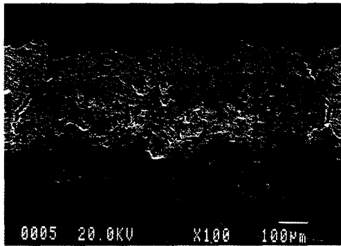
Fig. 7 Plasma-sprayed ZrO_2-8\%Y_2O_3 coating showing vertical cracks
